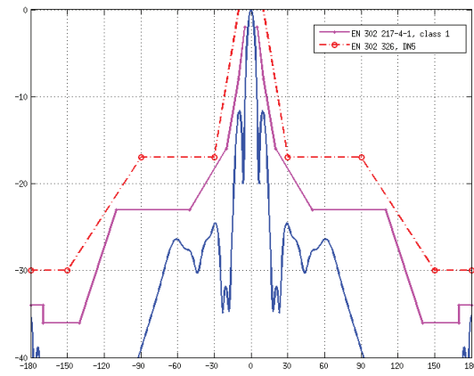
E-Plane Specs
