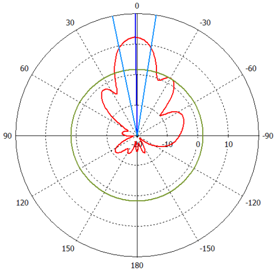
VP elevation
